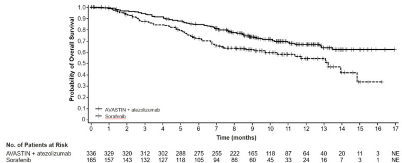
Figure 10: Kaplan-Meier Plot of Overall Survival in IMbrave150
